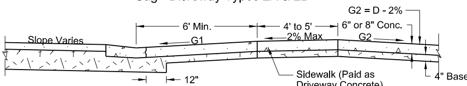
Summit - Driveway Types 2A & 2B
