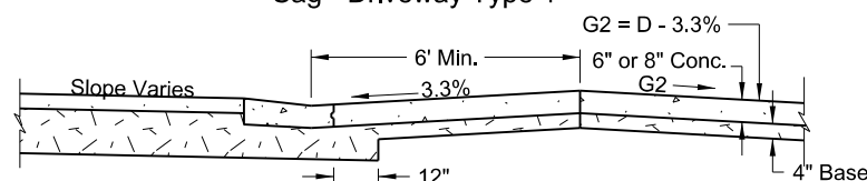
Summit - Driveway Type 1
