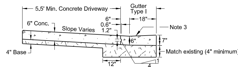
6" Section B-B
