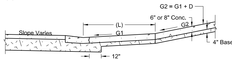
Sag - Driveway Type 1
